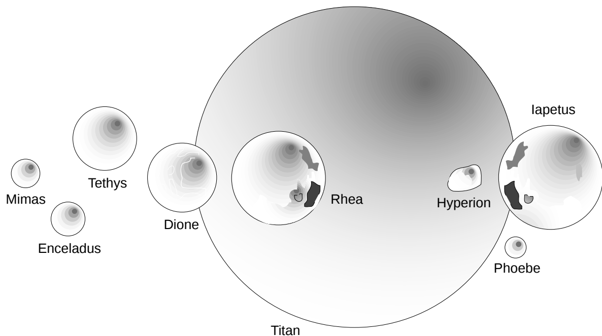
Saturn's major moons
